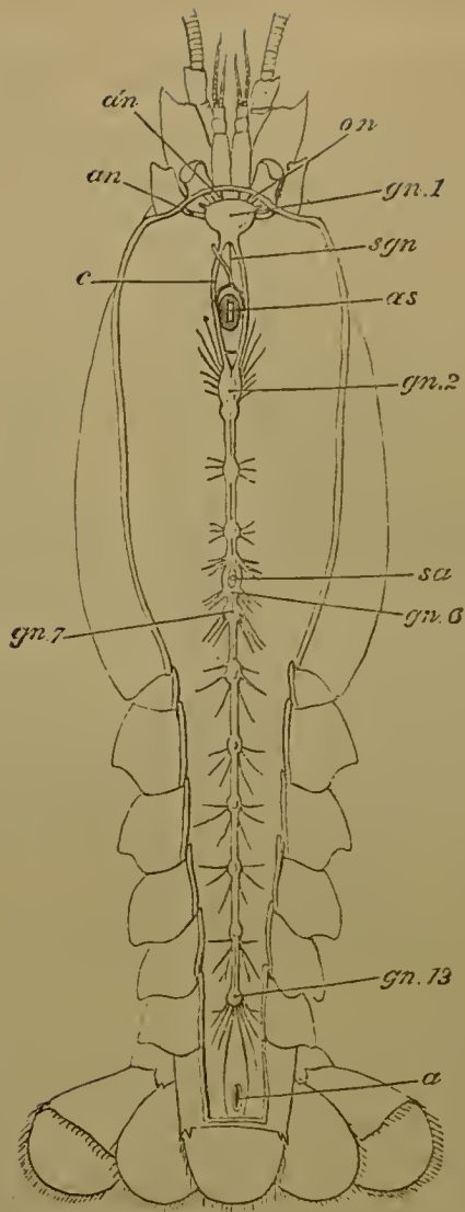
FIG. 25.— Astacus fluviatilis .—The central nervous system seen from above (nat. size). α , vent; an , antennary nerve; a'n , antennular nerve; c , circumoesophageal commissures; gn. 1 , supraoesophageal ganglion; gn. 2 , infraoesophageal ganglion; gn. 6 , fifth thoracic ganglion; gn. 7 , last thoracic ganglion; gn. 13 , last abdominal ganglion; æs , oesophagus in cross section; on , optic nerve; sa , sternal artery in cross section; sgn , stomatogastric nerve.
